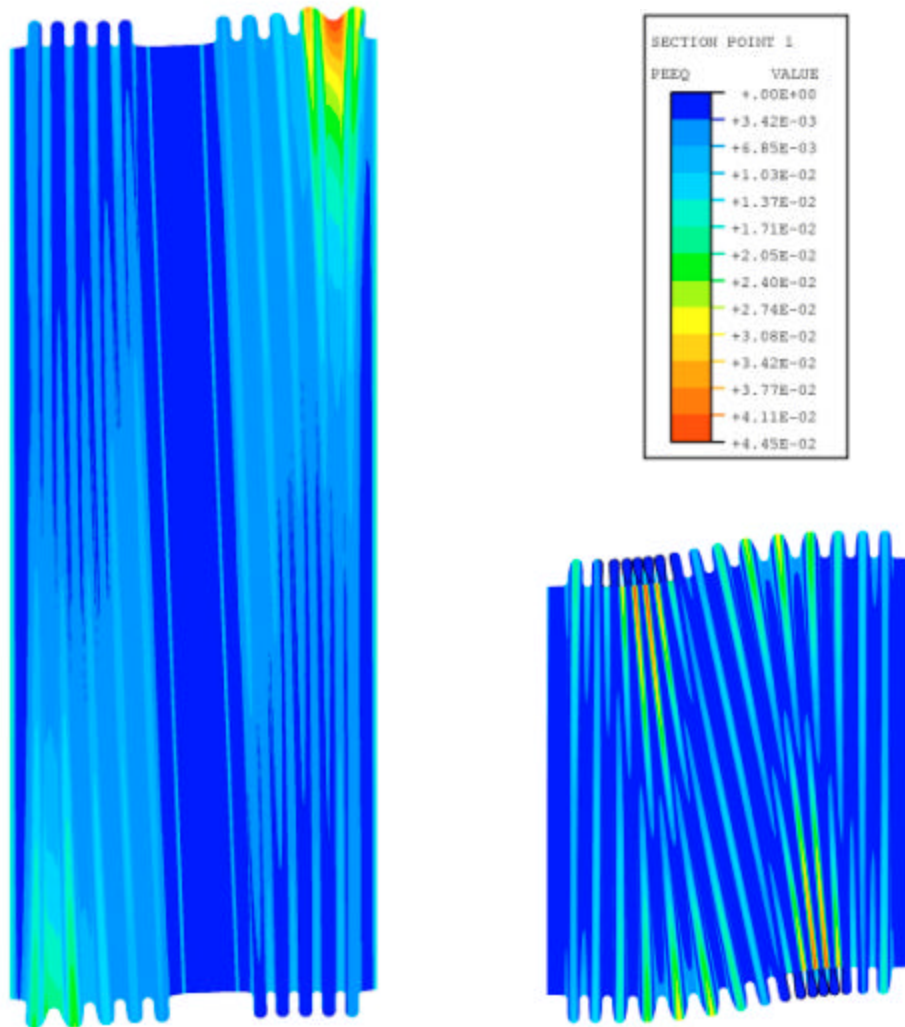
Figure 5 Shape and equivalent plastic strains at failure for median properties
