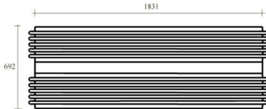
Figure 2 Vent line bellows (dimensions in mm)
