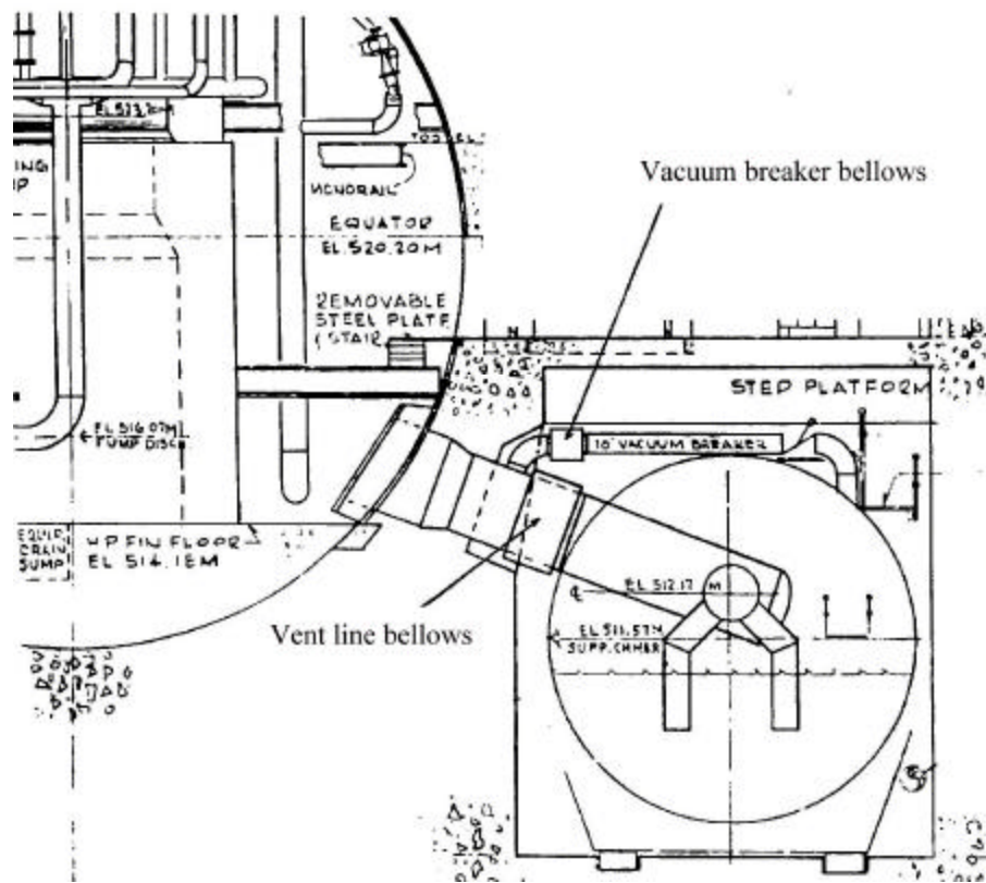
Figure 1 Bellows position
