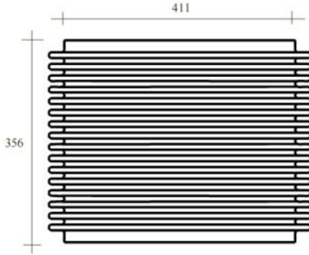
Figure 3 Vacuum breaker bellows (dimensions in mm)
