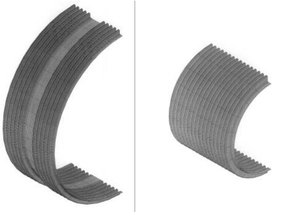
Figure 4 Finite element models for vent lines (left) and vacuum breaker lines (right)
