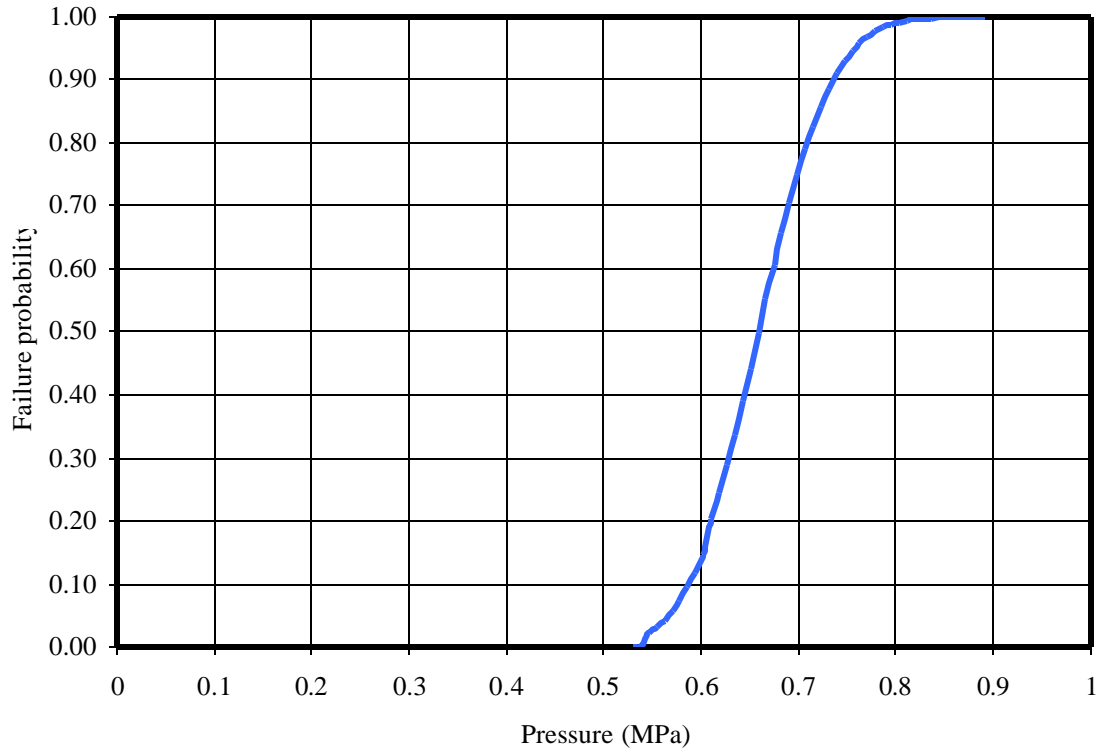
Figure 6 Fragility curve of the containment
